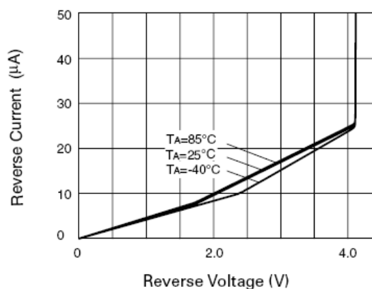
Reverse Characteristics
